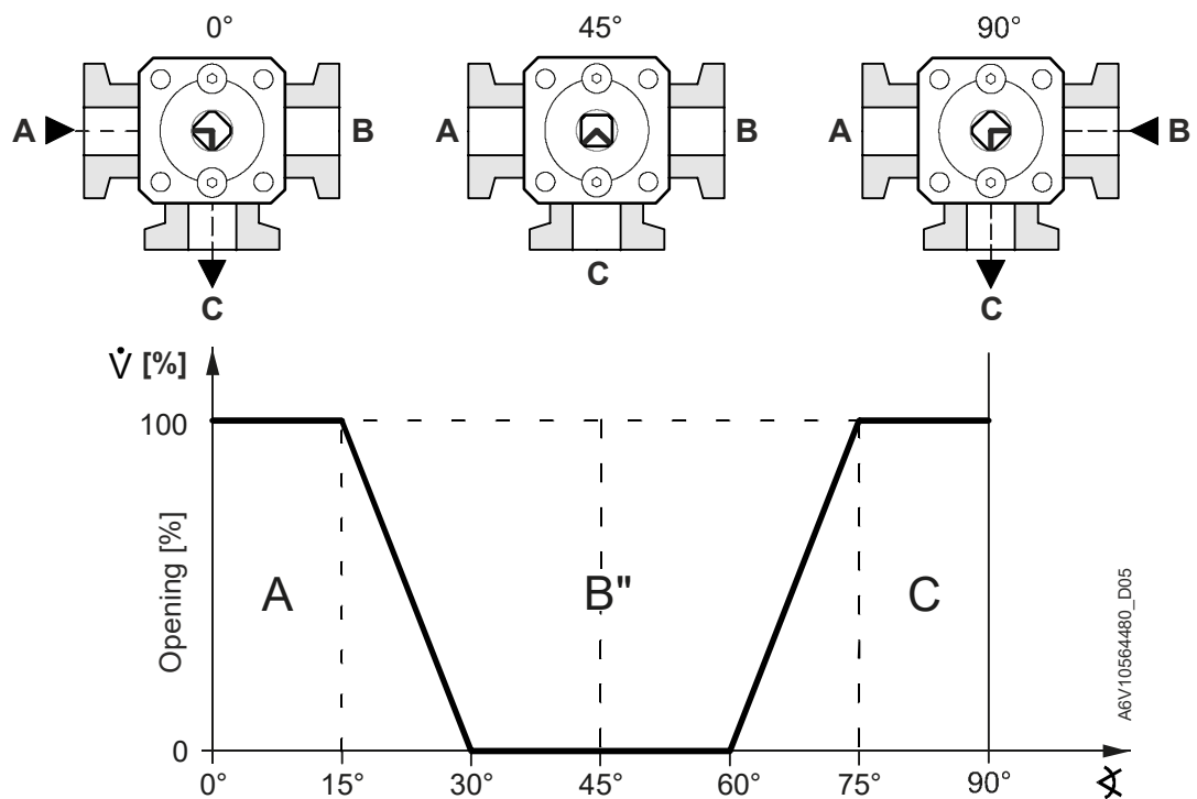
Ball valve characteristic curve DN10
