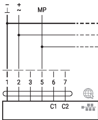
M-Bus parallel Modbus TCP or BACnet IP with PoE
