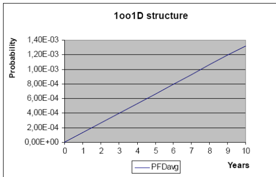
Fig. 17. Test Intervals and PFD avg
