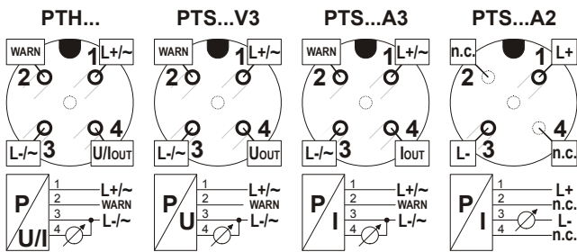
Fig. 16. Pin assignment of A-coded M12 plug
