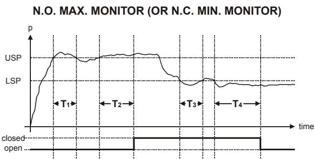
Fig. 7. DCM Switch output (max./min./window monitor)
