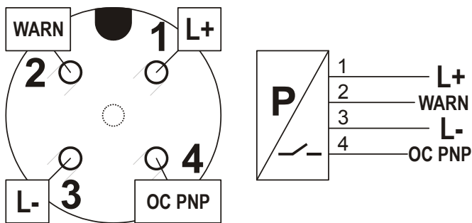
Fig. 6. Pin assignment of A-coded M12 plug
