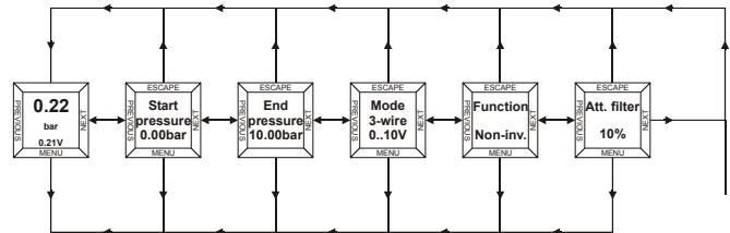
Fig. 12. DISPLAY LEVEL (example: SN 3-Wire)
