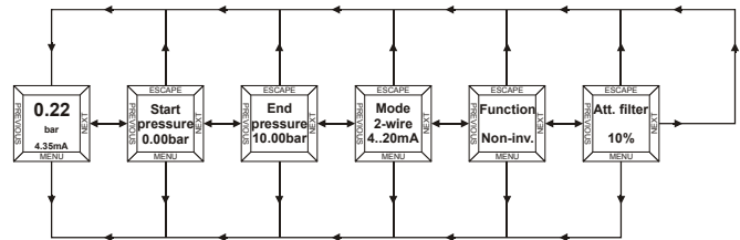
Fig. 11. DISPLAY LEVEL (example: SN 2-Wire)
